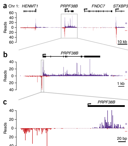
Figure 5 | DNA strand-specific Pol II occupancy at a representative region of the human genome, as determined by human NET-seq. (a–c) Pol II density for HeLa S3 cells is shown at different zoom levels for multiple genes (a), for a single gene (b) and for the promoter-proximal region of the gene shown in b (c). The Pol II density at the positive (+) and negative (–) DNA strand is shown in violet and red, respectively. The transcription start site and the direction of transcription is indicated by a black arrow. Exonic and intronic regions are shown as black boxes and lines, respectively. Adapted with permission from Mayer et al. 29 . HENMT1, HEN1 methyltransferase homolog 1; PRPF38B, pre-mRNA processing factor 38B; FNDC7, fibronectin type III domain containing 7; STXBP3, syntaxin binding protein 3.
