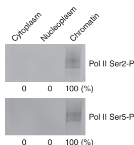
Figure 2 | Representative western blot showing the quantitative purification of elongating RNA Pol II by cell fractionation. Subcellular fractions have been obtained from \sim 1 \times 10^7 HeLa S3 cells. Sample volumes have been adjusted to the cytoplasmic fraction (largest volume) so that the western blot signals between the different fractions can be compared. The subcellular fractions have been probed with antibodies directed against the Pol II CTD Ser2-phosphorylated (top; 3E10 antibody) and CTD Ser5-phosphorylated form (bottom; 3E8 antibody). The numbers below the blots represent the western blot signals in percentages, as obtained by image quantification using ImageJ 1.47v software 64 . The full-size blots of the western analysis are shown in Supplementary Figure 2 . P, phosphorylated.
