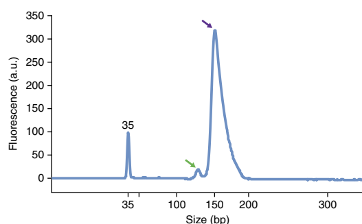
Figure 4 | Bioanalyzer electropherogram of a representative human NET-seq library. The NET-seq library was generated from 3 \mu\text{g} of RNA obtained from HeLa S3 cells. Approximately 1.1 ng of the final NET-seq library was loaded onto a high-sensitivity DNA microfluidic chip. The profile shows a prominent peak around 150 nt (violet arrow) and a smaller peak around 120 nt (green arrow). The less prominent peak corresponds to background that arises from unextended RT primer leading to a 119-nt PCR product (see also Fig. 3c,d ). This background DNA also results in sequencing data. However, these sequencing reads will contain sequences of the 3' and 5' linker regions that are part of the RT primer and are computationally removed. The background DNA should be lower than 10%, as compared with the amount of the NET-seq library. The peak at 35 nt represents the manufacturer's internal standard. a.u., arbitrary units.
